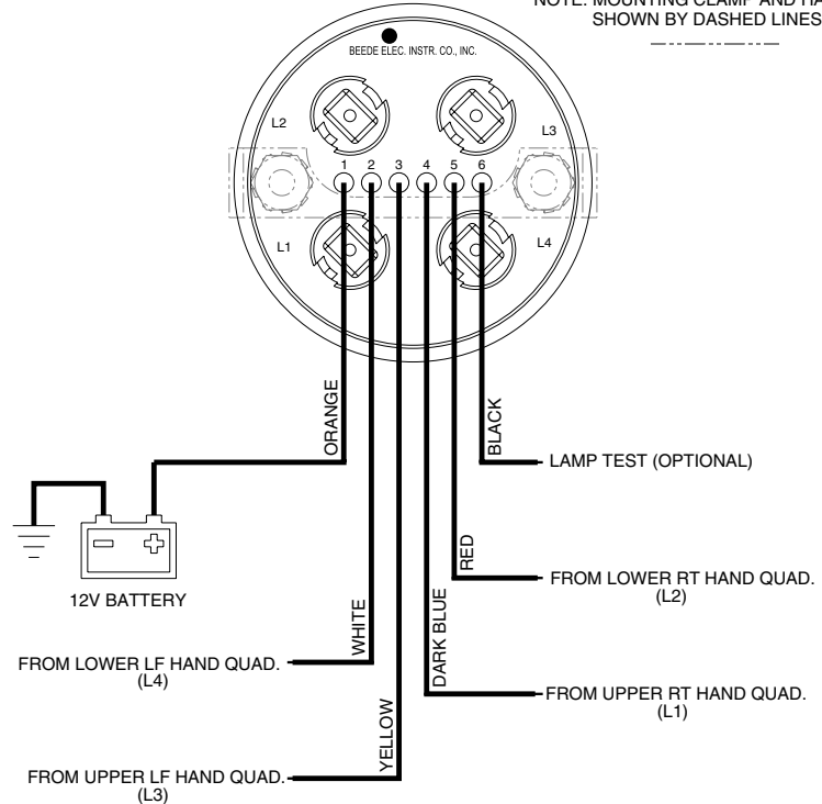
WARNING GAUGE (REAR VIEW)
